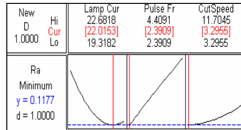
Fig. 2 Optimization results of surface roughness.
